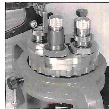
Precision 5-Hole Turret with 20 locking lugs takes just seconds to change.
